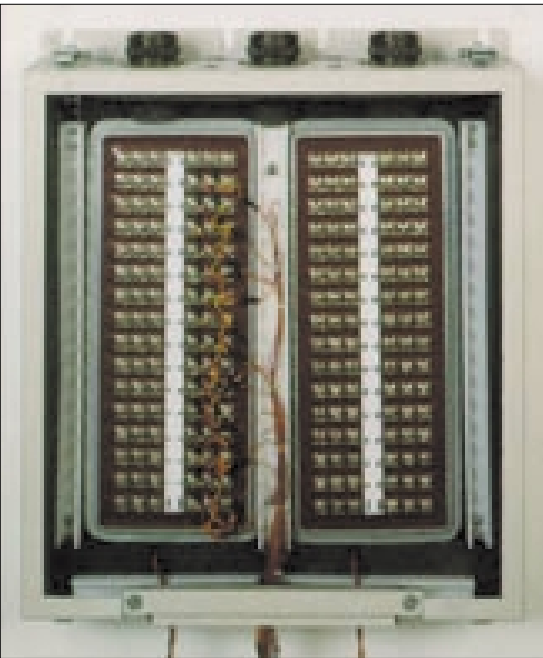
View of a 64-channel UTR. Kaye has also supplied custom UTR's, such as 64-channel units, some with special connectors and water cooling tubes. Custom UTR's have been developed for Rolls-Royce, Arnold Air Force Base, General Electric and Pratt & Whitney.
