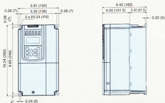
Main body of standard inverter (7.5HP or smaller) Unit:inch (mm)
