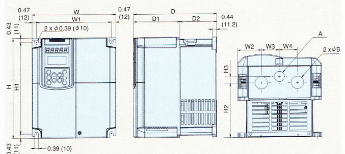
Main body of standard inverter (10 to 40HP) Unit:inch (mm)
