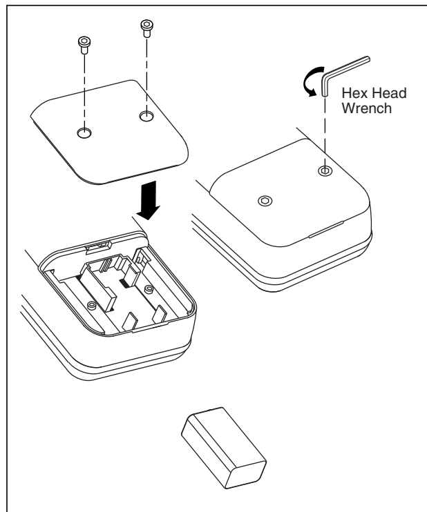
Figure 7. Battery Replacement
