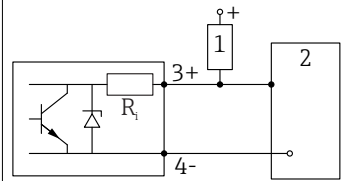
10 Connection of a digital input
