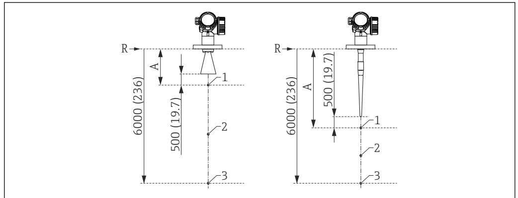
40 Points of the 3-point linearity protocol; Dimensions: mm (in)
