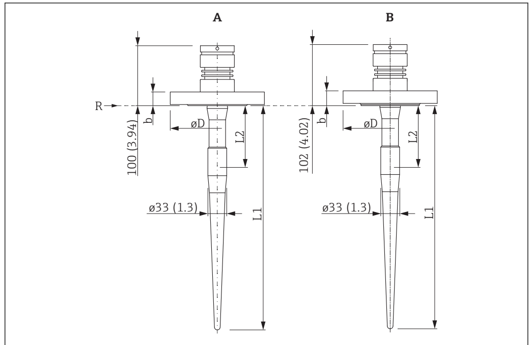
27 FMR53 with flange; dimensions: mm (in)
