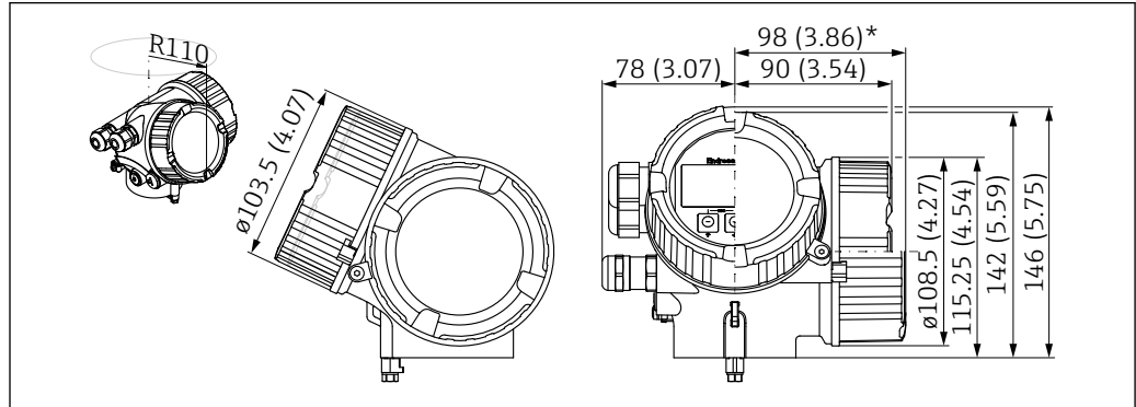
24 Housing GT18 (316L); Dimensions in mm (in) *for devices with integrated overvoltage protection.
