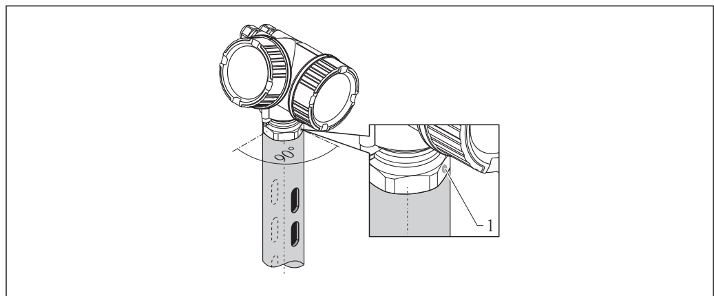
19 Installation in stilling well
