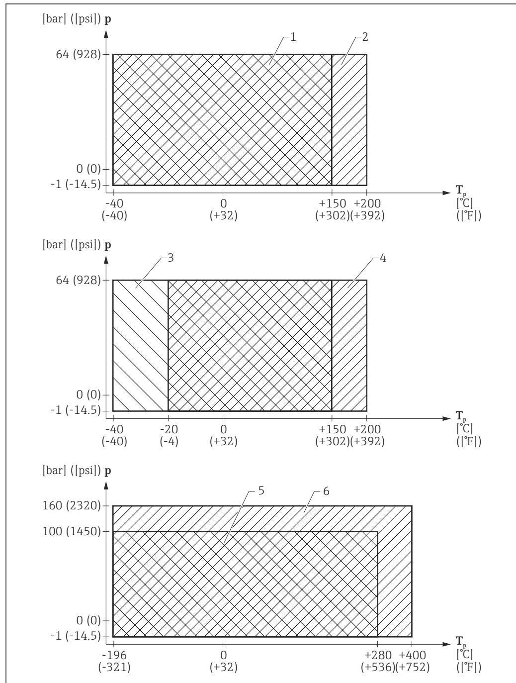
22 FMR54 with horn antenna: Admissible range of process temperature and process pressure
