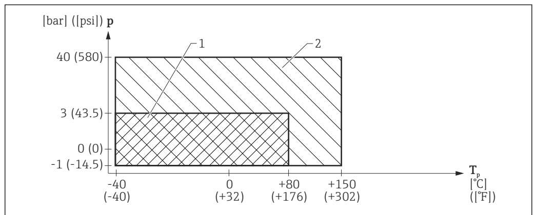
21 FMR53: Admissible range of process temperature and process pressure
