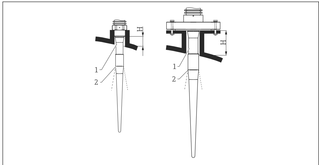
17 Nozzle height and diameter for the rod antenna (FMR53)
