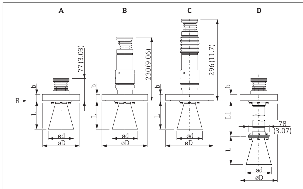
29 FMR54 with horn antenna; dimensions: mm (in)
