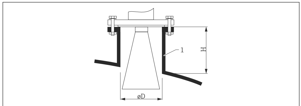
18 Nozzle height and diameter for the horn antenna (FMR54)
