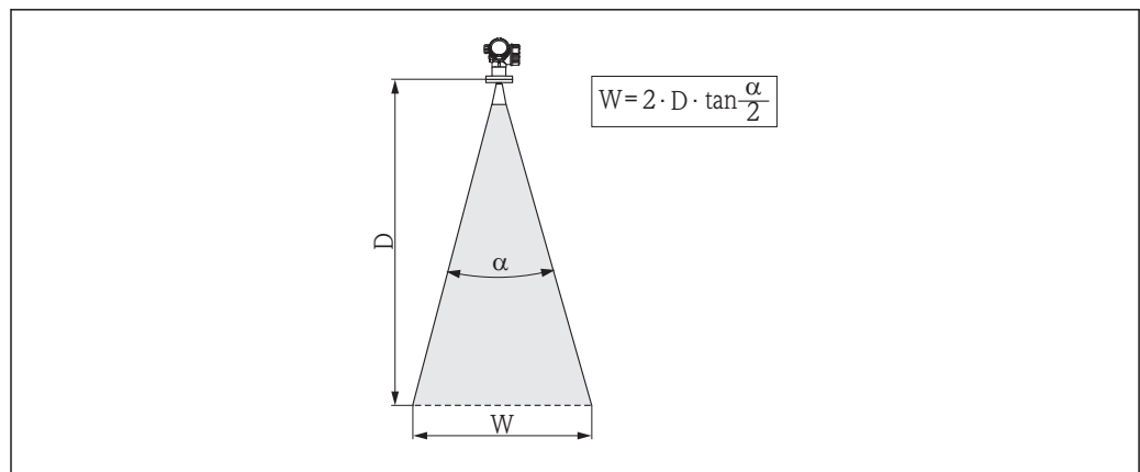
16 Relationship between beam angle \alpha , distance D and beamwidth diameter W
