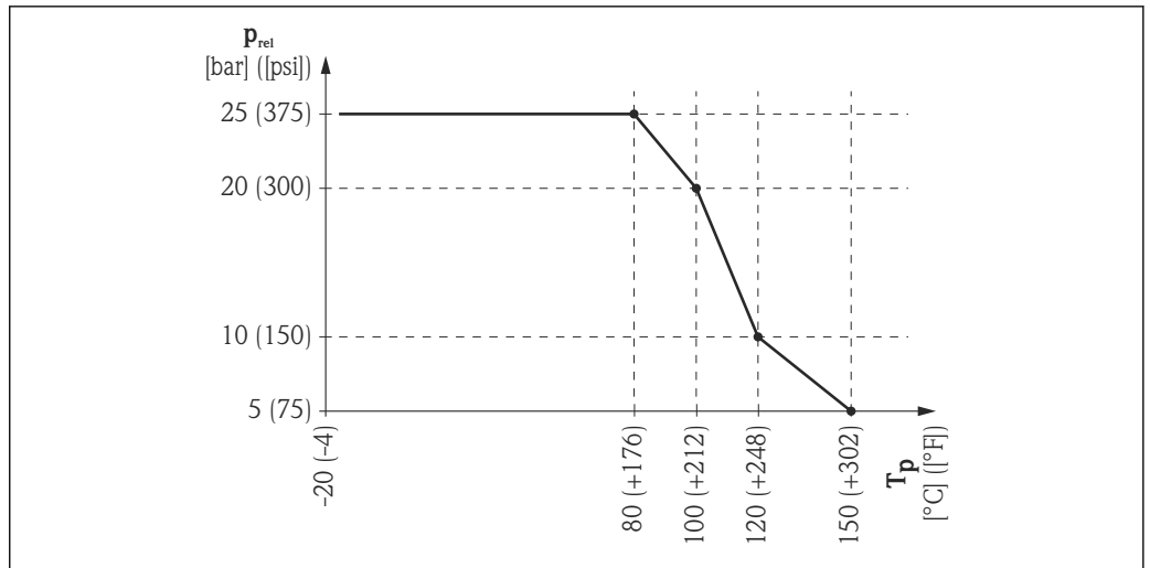
23 FMR54 with planar antenna: Admissible range of process temperature and process pressure
