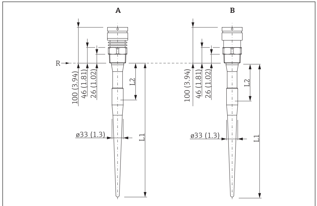
28 FMR53 with thread; dimensions: mm (in)
