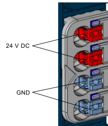
Connector Block
