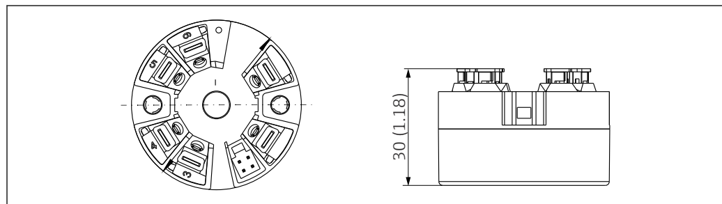
5 Version with spring terminals. Dimensions are identical to the version with screw terminals, apart from housing height.
