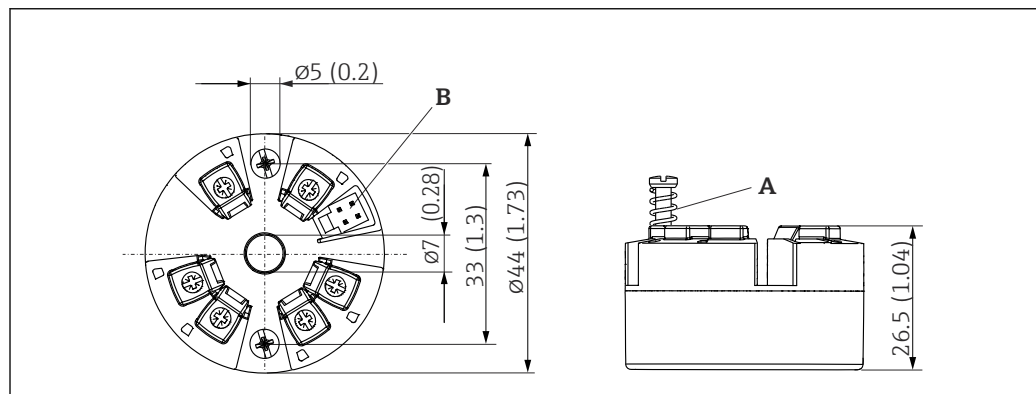
4 Version with screw terminals
