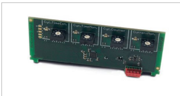
Monitoring board for on/off operation (EA25-250)
