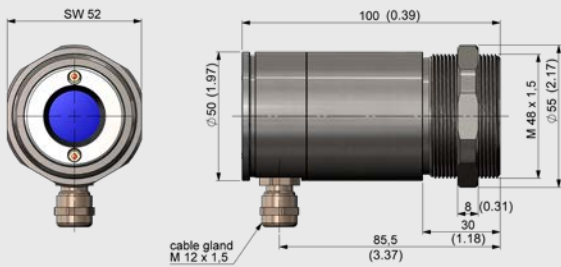
Sensing head
