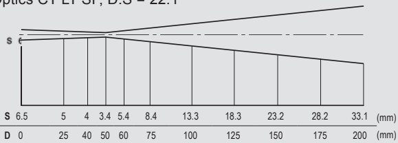
Optics CT LT SF, D:S = 22:1
