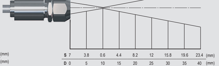
Optics CT LT CF, D:S = 22:1 (far field = 1.5:1)
