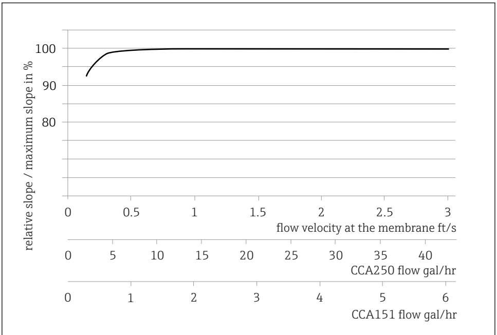
3 Correlation between slope of electrode and flow velocity at the membrane/volume flow in assembly
