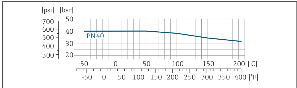
24 With flange material: 1.4539 (904L), Alloy C22; lap joint flanges (not wetted) 1.4404 (316/316L)
