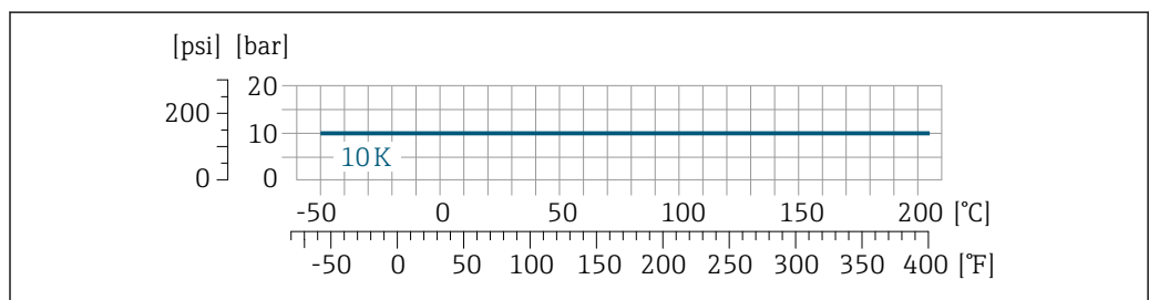
26 With flange material: 1.4539 (904L); lap joint flanges (not wetted): 1.4404 (316/316L)
