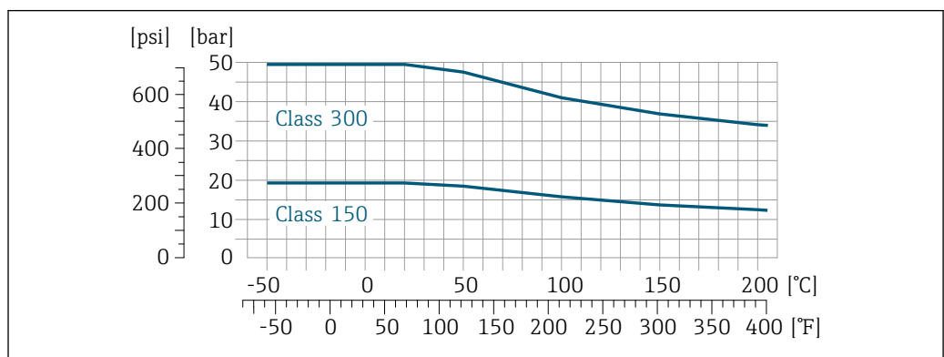
25 With flange material: 1.4539 (904L); lap joint flanges (not wetted) 1.4404 (316/316L)
