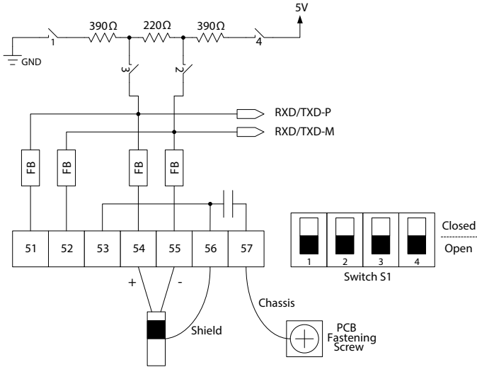
Figure 4: Signal wiring diagram
