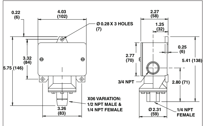
B400 Dimension Drawing – 70A1084
