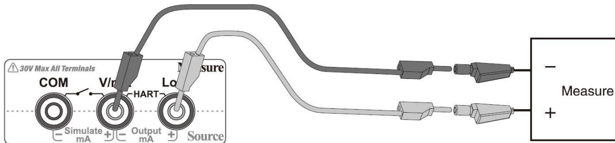
Figure 12 Current Output
