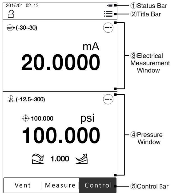
Figure 7 Main Screen
