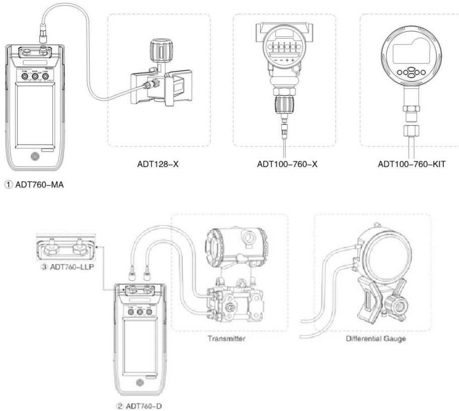
Figure 8 Output Connection
