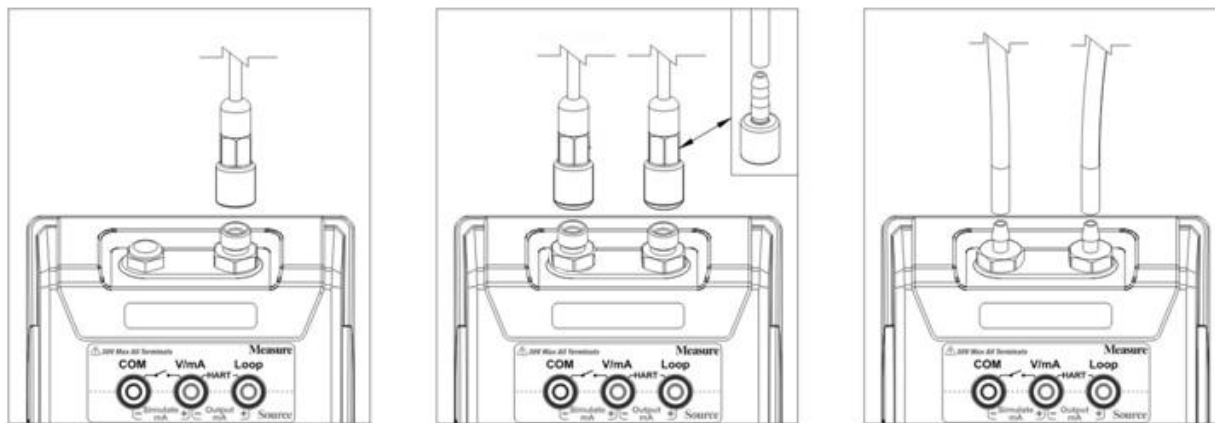
Figure 6 Pressure Connection
