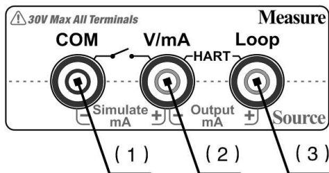
Figure 5 Electric Connection
