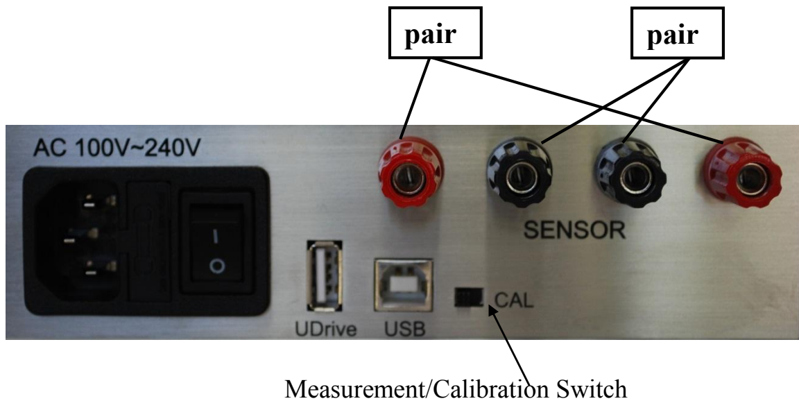
Figure 3: Rear Panel and Sensor Terminals
