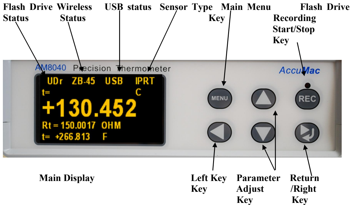
Figure 1: Front Panel
