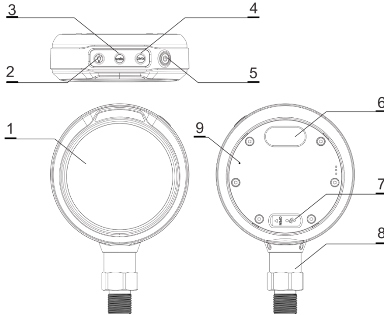
Figure 1 Basic Structure
