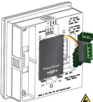
3-9900 Panel Mount Transmitter
