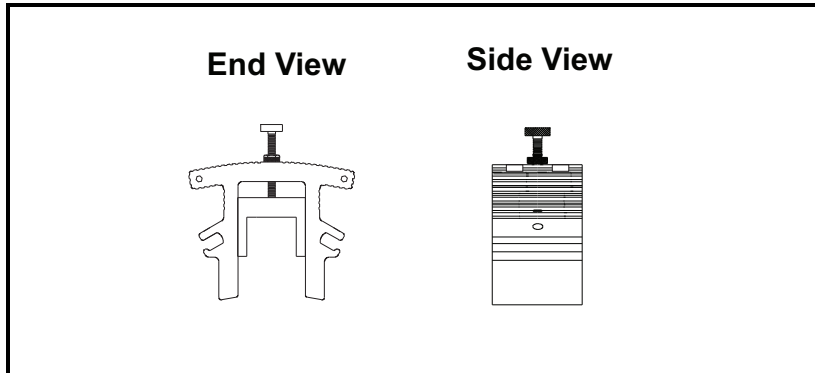
Figure 8: General Clamping Fixture Block
