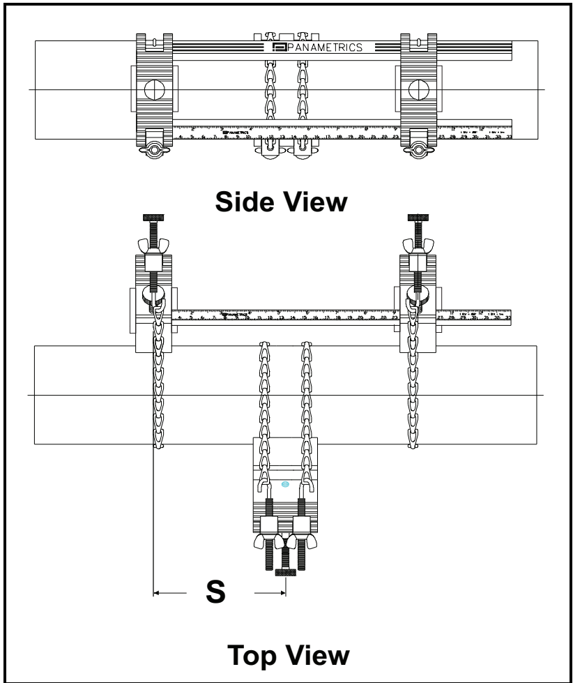
Figure 6: Single-Traverse Clamping Fixture w/o Transducers
