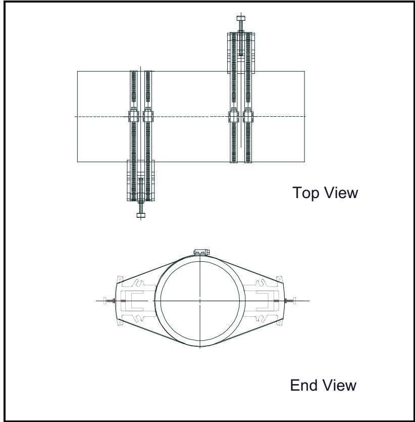
Figure 10: Single-Traverse GCF Installation w/o Transducers
