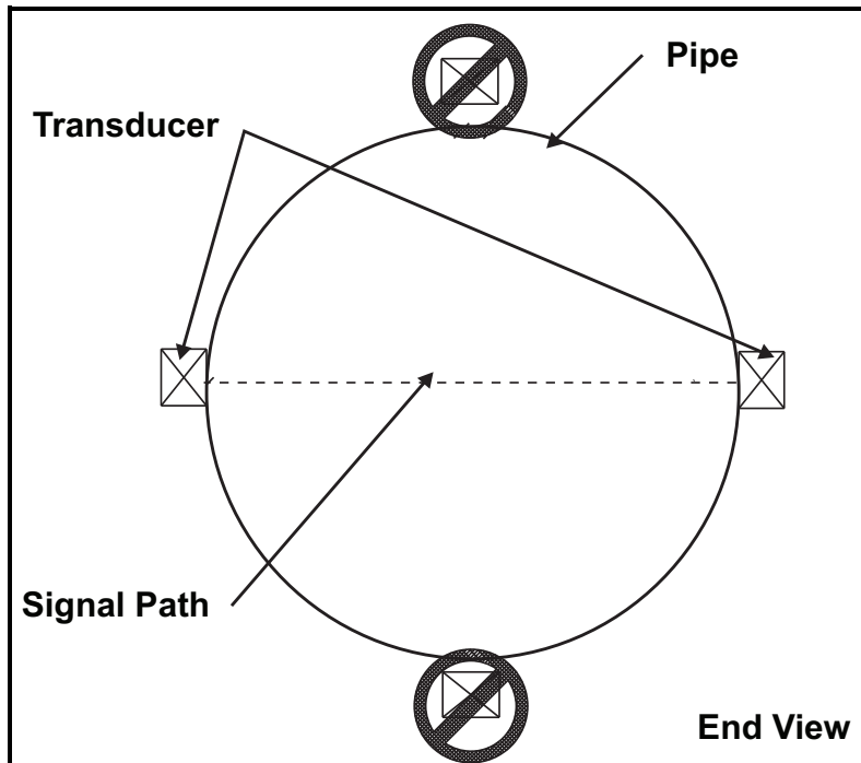
Figure 2: Transducer Placement
