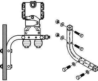
Panel mount (1)
