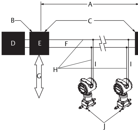
Figure 6. Wiring
