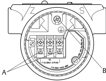
Figure 5. Terminals
