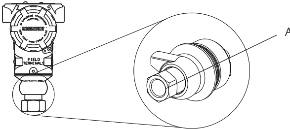
A. Low side pressure port (atmospheric reference)
