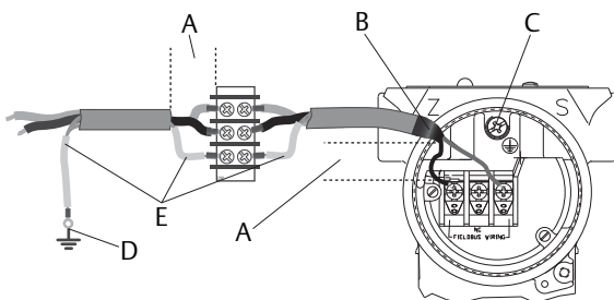
Figure 7. Wiring
