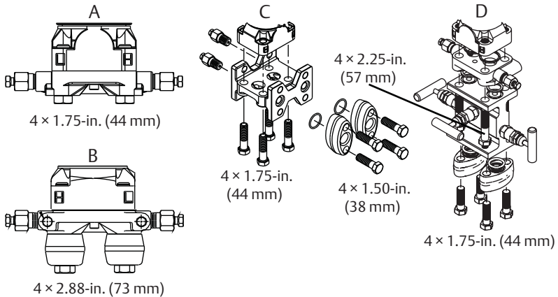
Figure 1. Common Transmitter Assemblies
