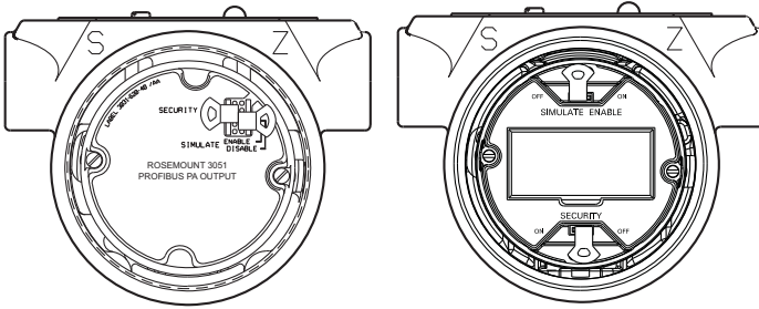
Figure 4. Transmitter Jumper Locations
