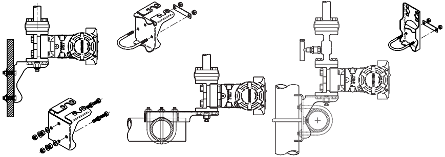
Rosemount 3051T
