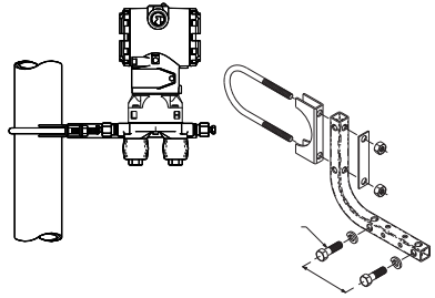
Pipe mount
