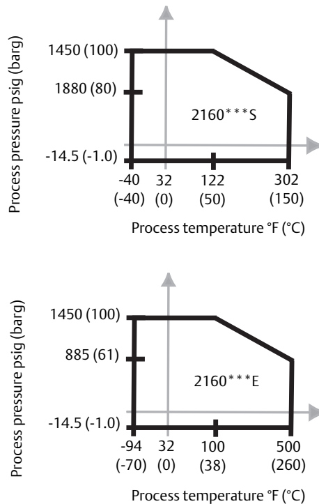
Figure 1. Operating Pressures
