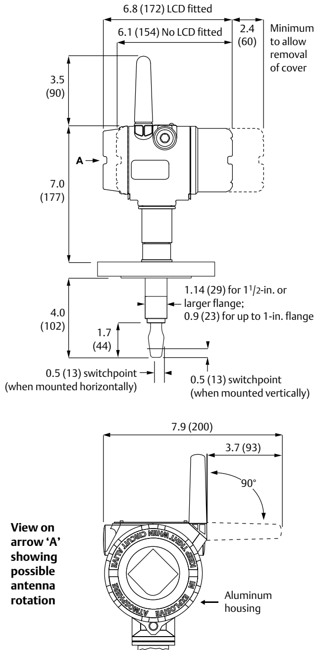
Figure 5. Flanged Process Connections (Standard Length Fork)
