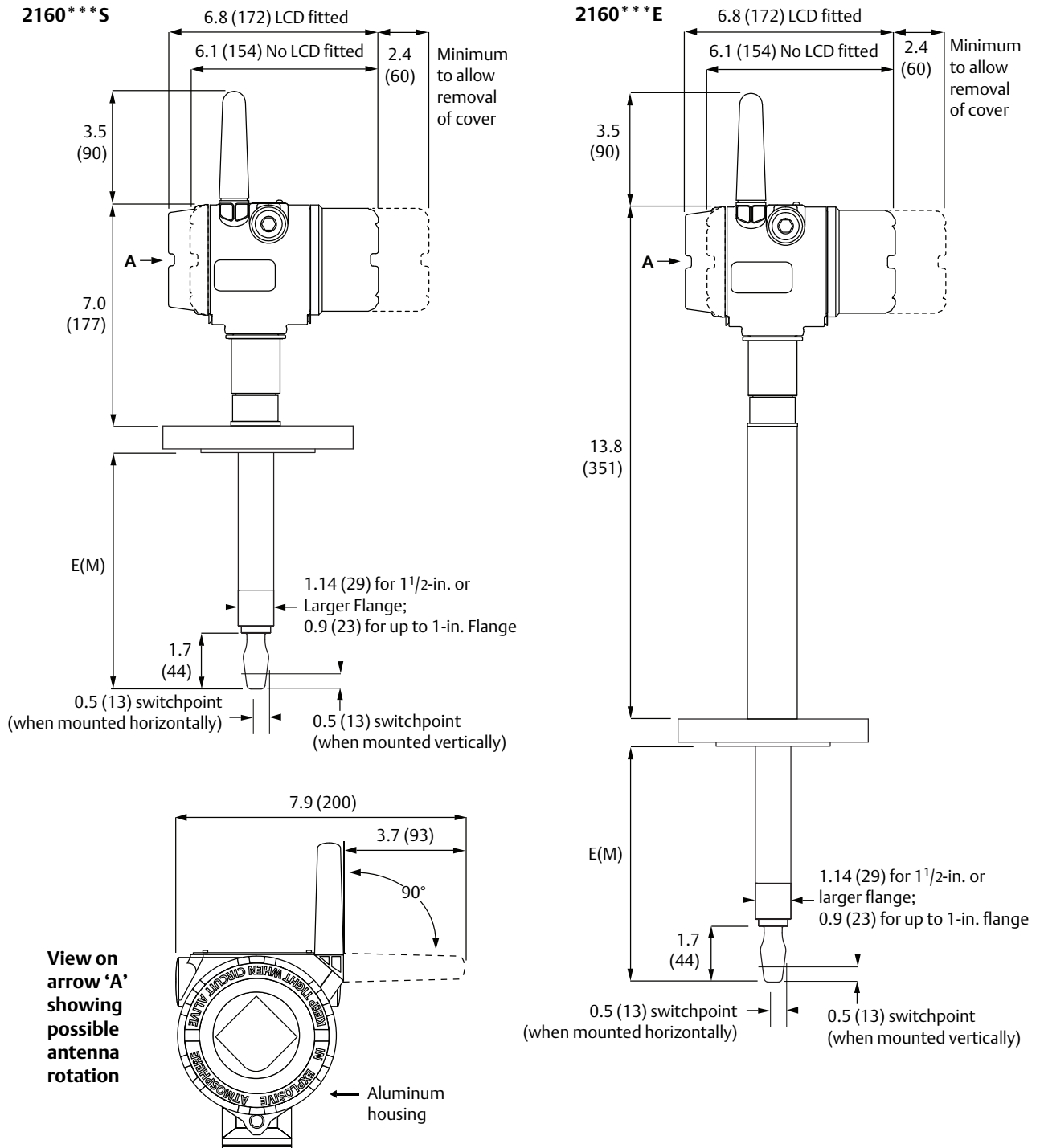
Figure 6. Flanged Process Connections (Extended Length Fork)
