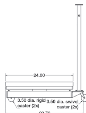
Caster Model
